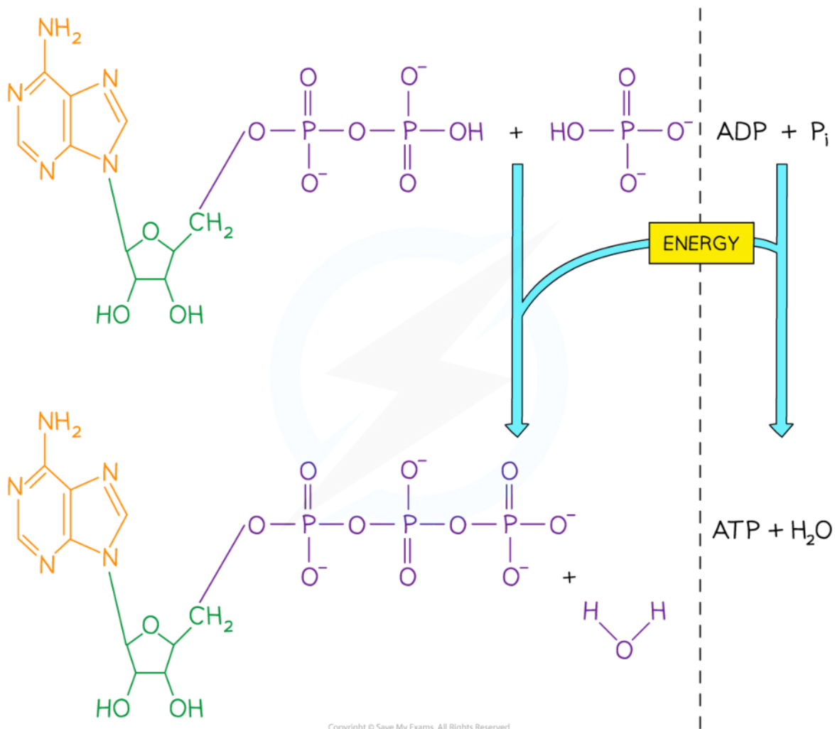
Energy-requiring synthesis of ATP from ADP and Phosphate
