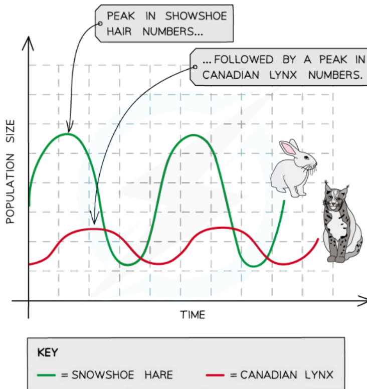
An example of a graph used to model a predator-prey cycle between the Canadian lynx and the snowshoe hare
