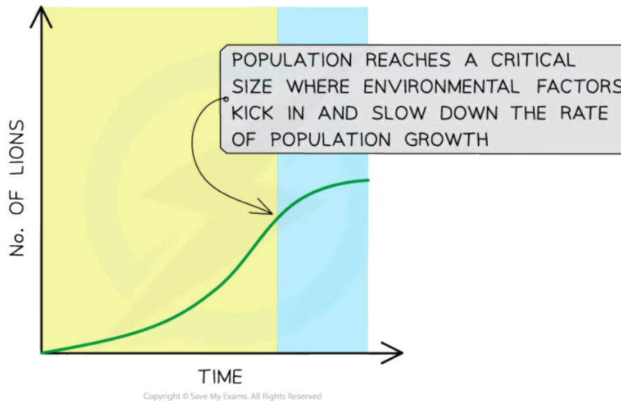
An example graph showing the population growth of a population of lions and the point at which the carrying capacity of this population has almost been reached
