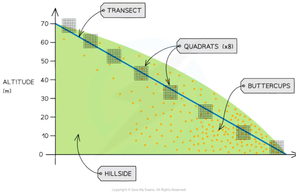
An example of a belt transect on a hillside—quadrat is placed at regular intervals (every 10 m of altitude gained) and the number of individuals (of the species being investigated e.g. buttercups) in each quadrat is recorded
