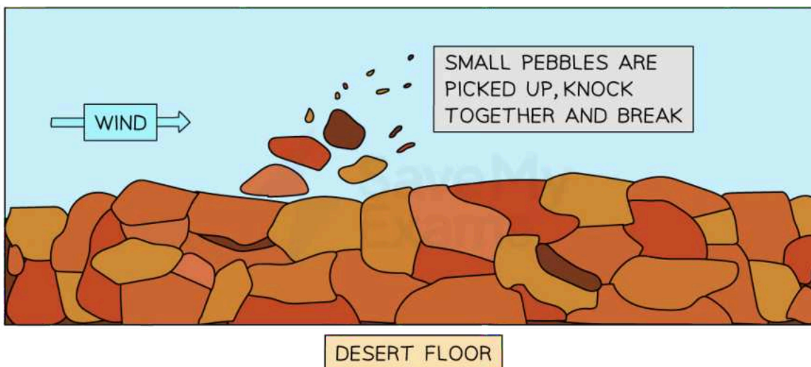
Image showing how desert attrition occurs
