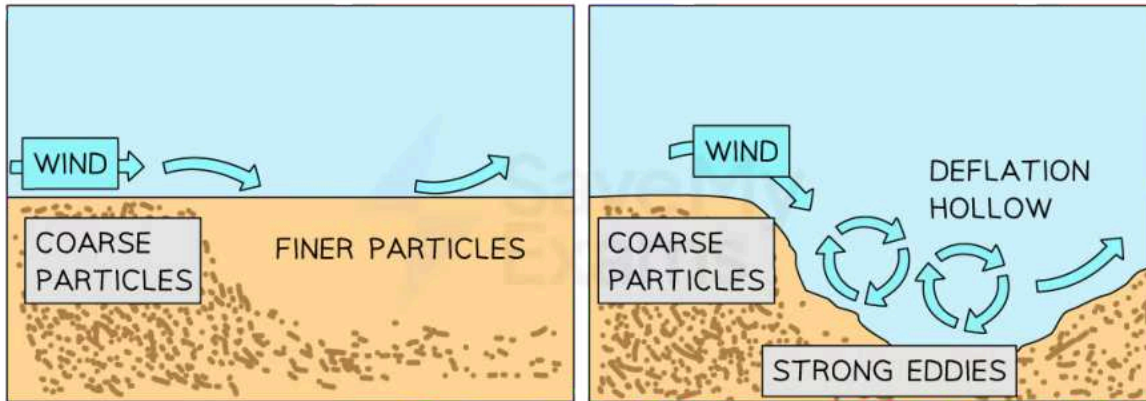
Image showing how deflation hollows form
