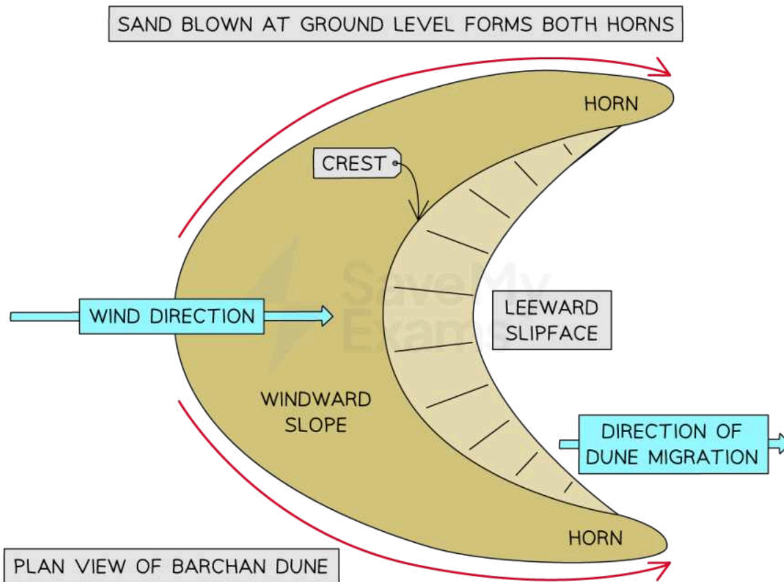
Diagram showing the characteristic features and formation of barchan dunes
