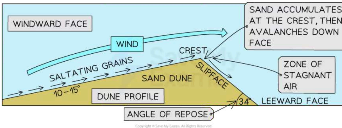
Image showing how a sand dune is formed, dependent on wind and loose sand.
