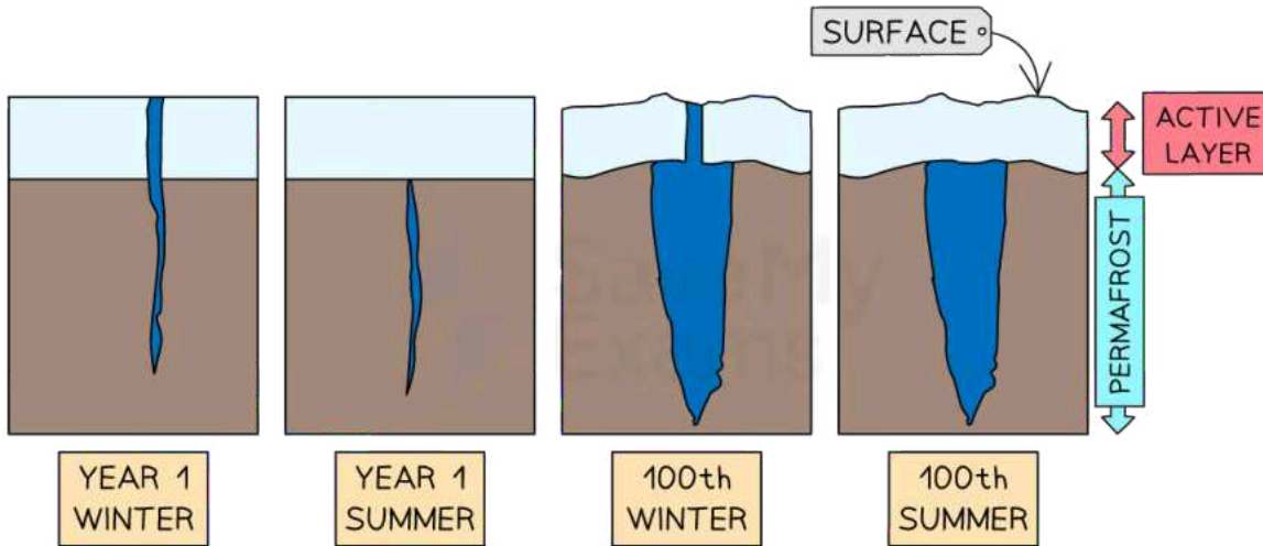
Ice wedge formation over time
