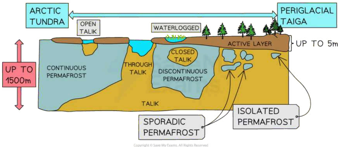
Image showing types of permafrost found in periglacial areas
