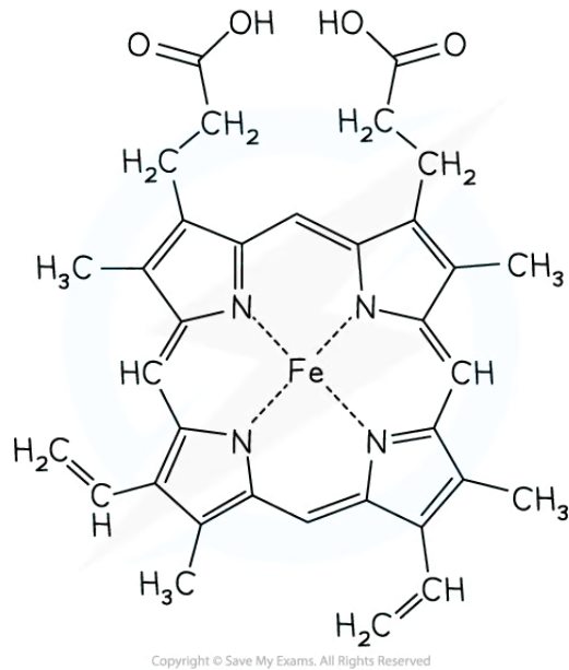
The structure of haem
