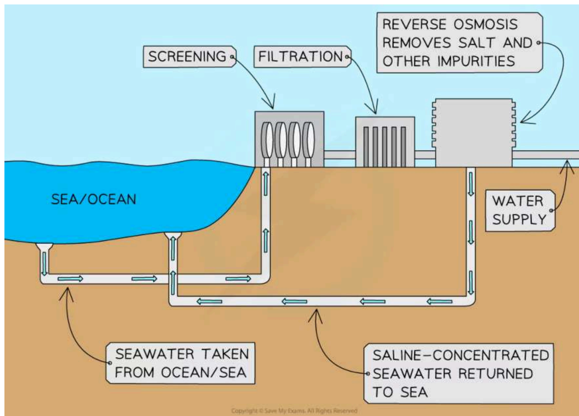
Desalination process
