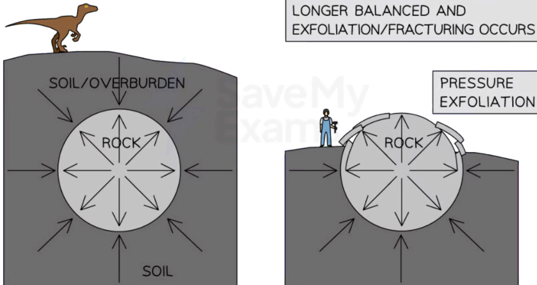
Image showing pressure release exfoliation over time
