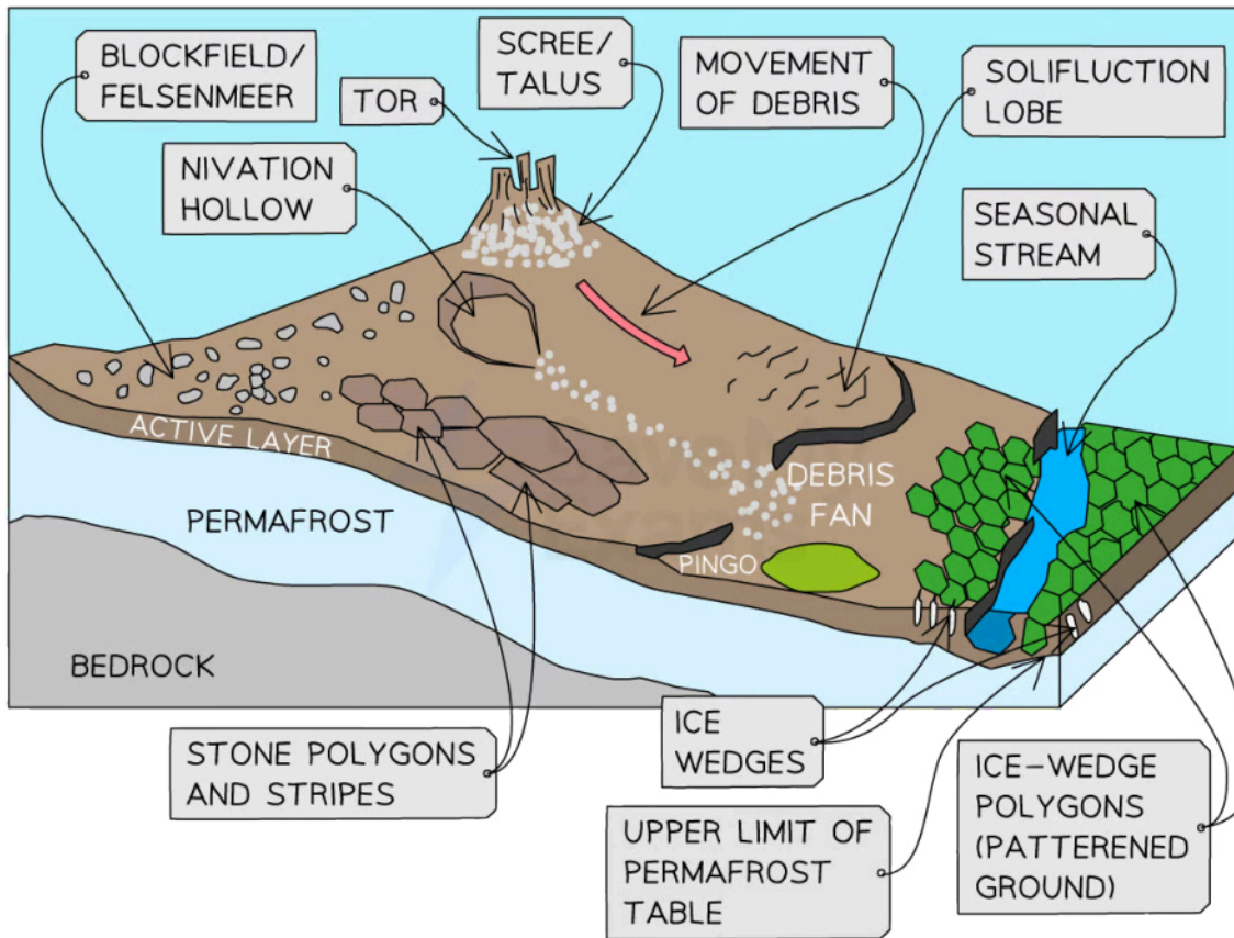
Image showing main features of a typical periglacial landscape
