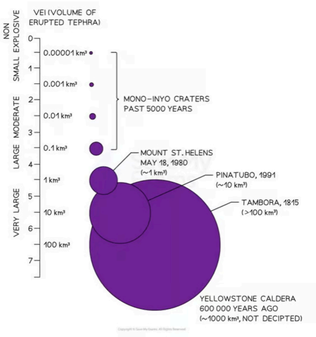
Volcanic Explosivity Index
