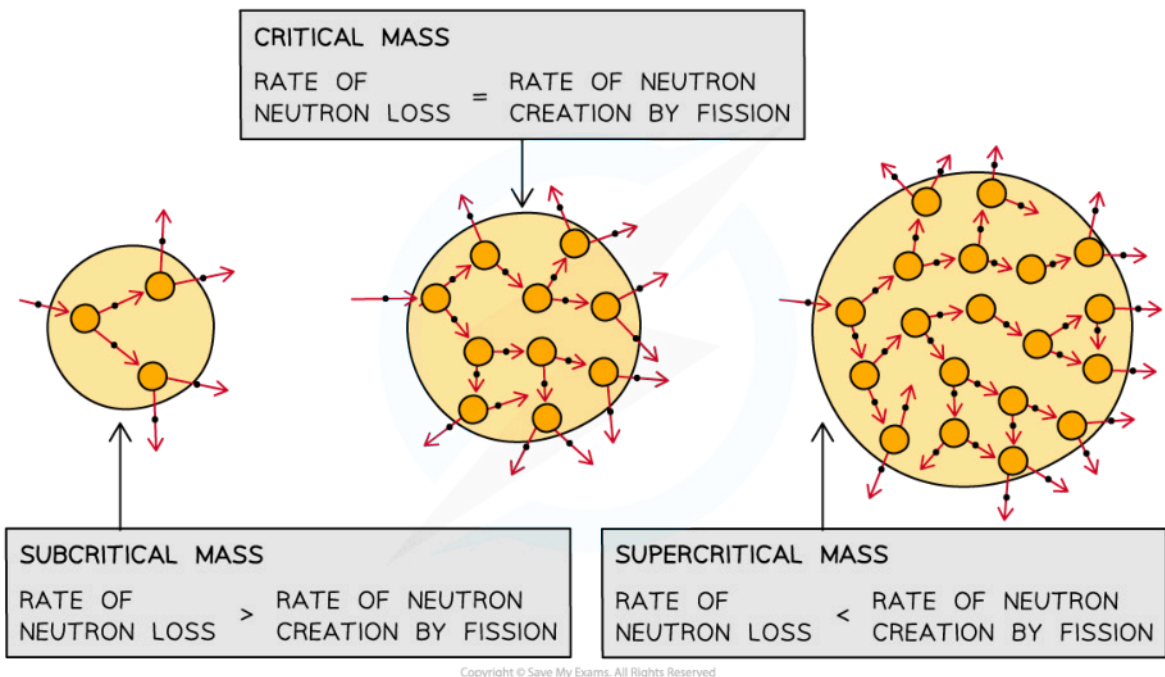
Subcritical, critical and supercritical mass
