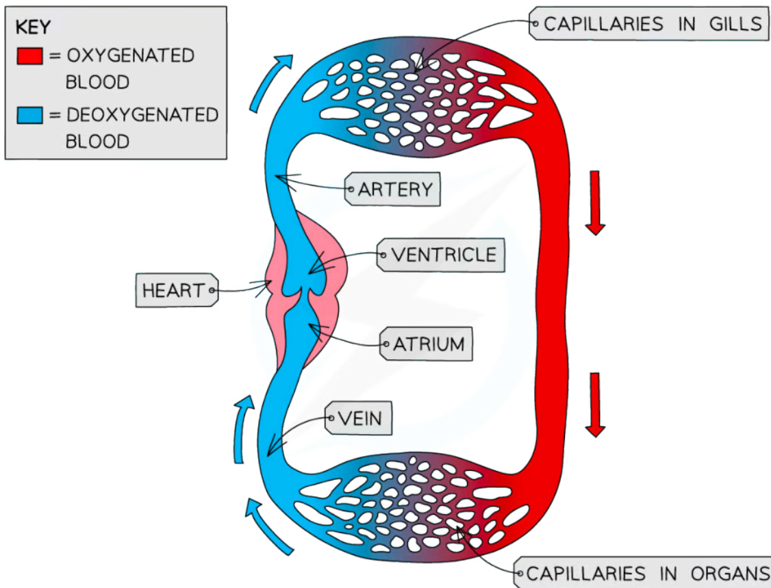
Bony fish have single circulation
