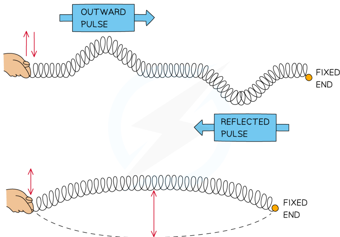
Formation of a stationary wave on a stretched spring fixed at one end
