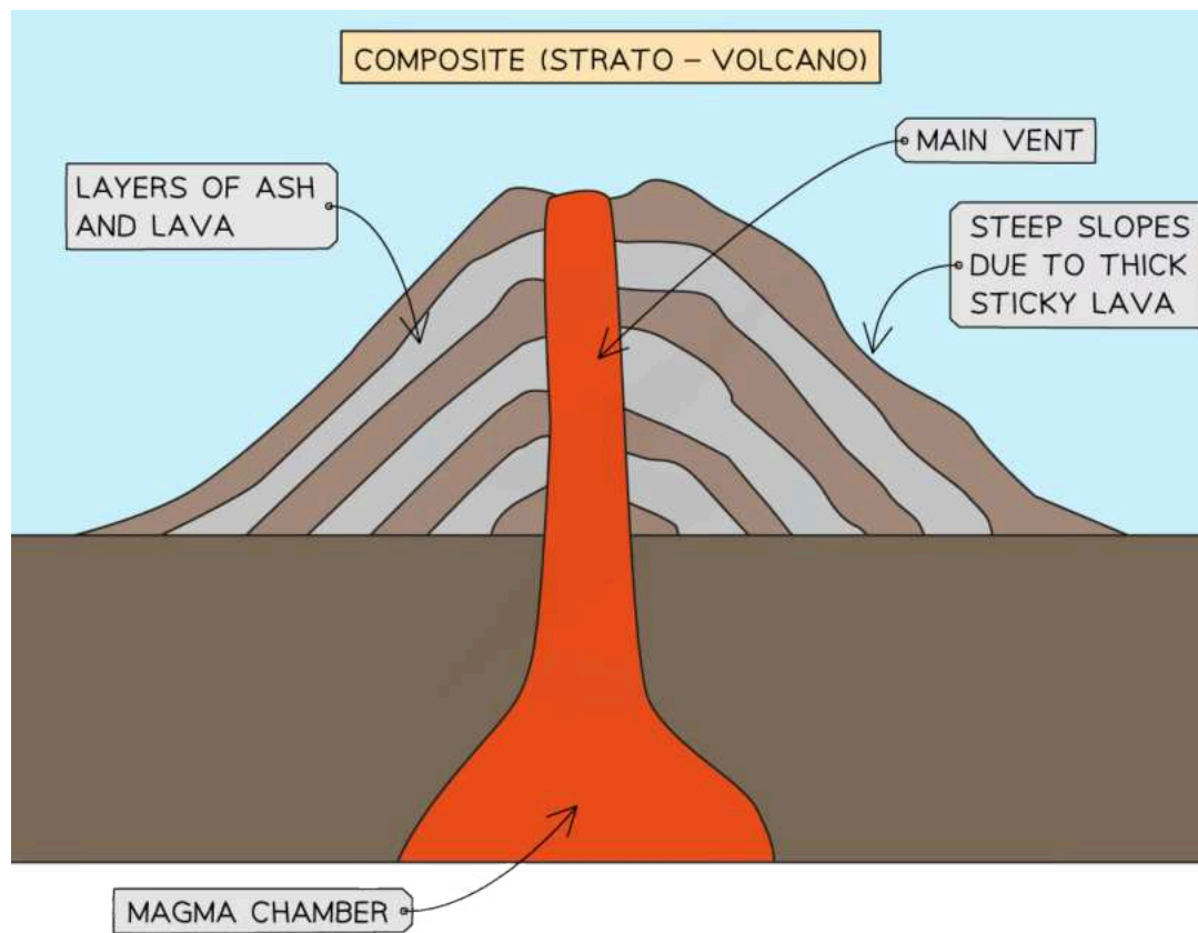
Composite volcano
