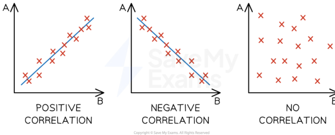
The main types of correlation between two variables
